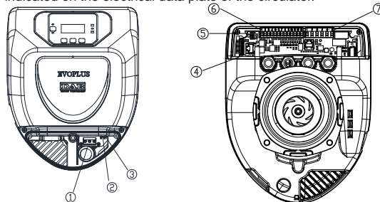
Figure 4: Electrical connections (front)
