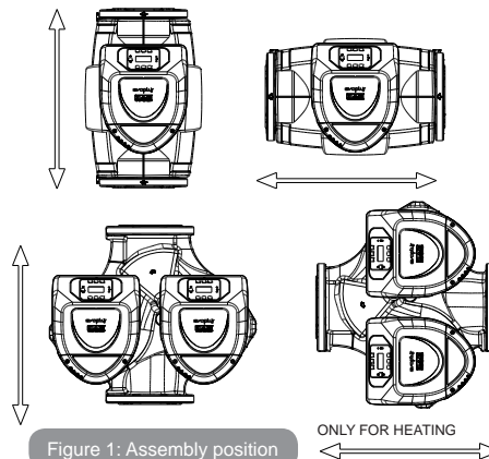
Figure 1: Assembly position
